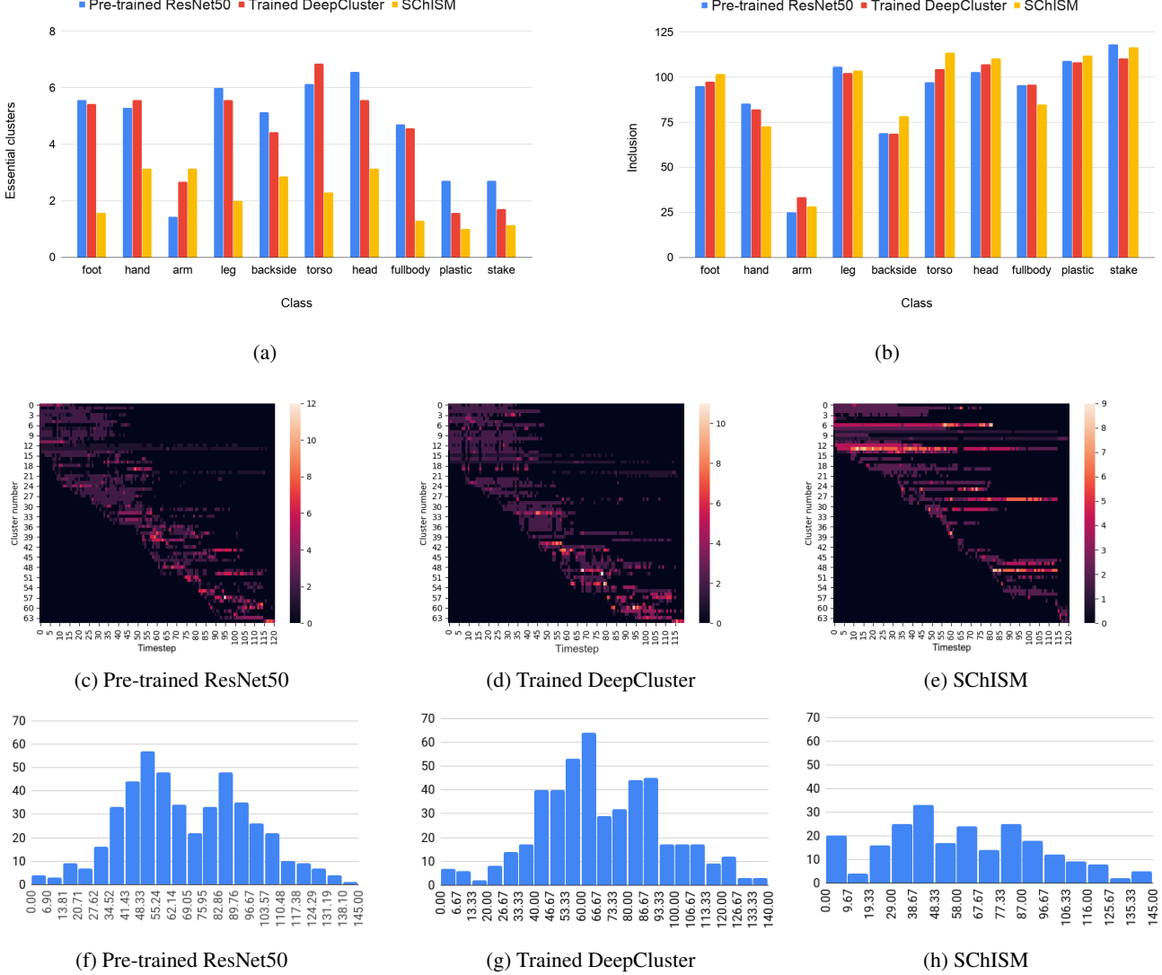
Figure 6: (a) and (b) compare pre-trained CNN-based image clustering, trained DeepCluster, and SchISM through the number of essential clusters and number of timesteps captured for each body part (inclusion). The plots show that SchISM was able to capture same or higher number of timesteps in smaller number of essential clusters. (c), (d) and (e) compare the clusters generated from the methods for one subject respectively through a visualization. Color indicates the number of images in each timestep and cluster. The plots indicate that SchISM generates clusters with longer sequences and with less gaps in timesteps compared to the other methods. (f), (g), and (h) show gap histograms for clusters and indicate that clusters generated using SchISM have minimum gaps compared to the other methods.
