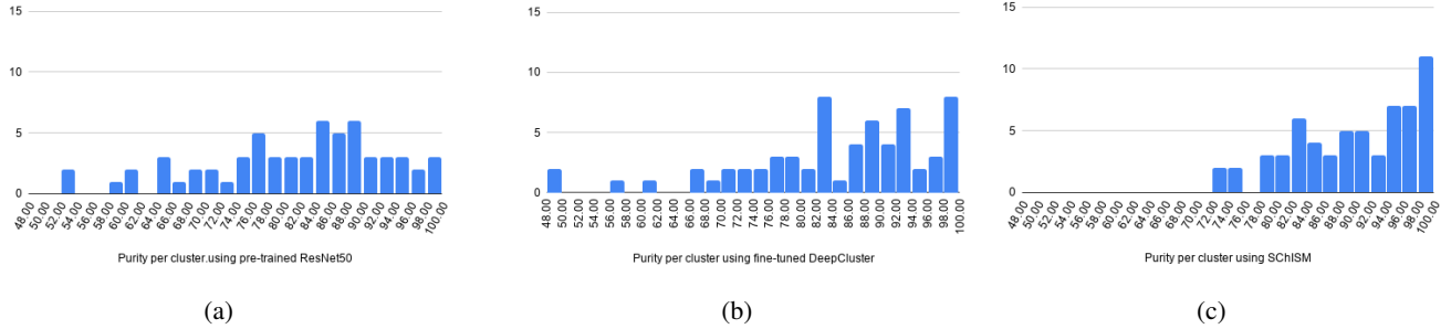
Figure 4: Purity histogram for the clusters from pre-trained CNN-based image clustering, trained DeepCluster and SchISM. The majority of the clusters obtained using SchISM have purities higher than 84% for the same number of clusters.
