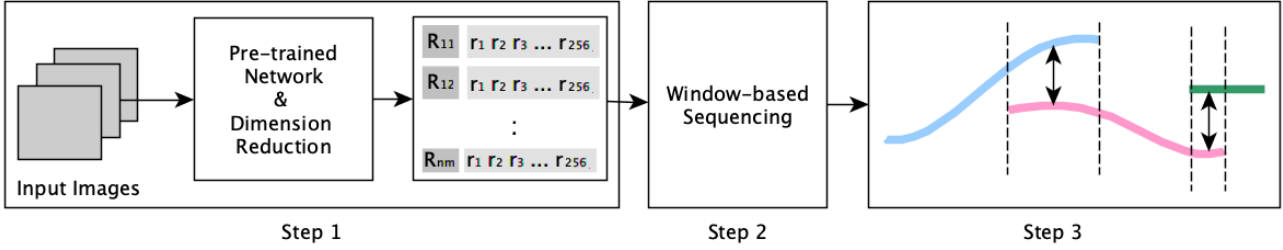
Figure 2: The overall architecture of our proposed method is shown. Step 1: Input images are mapped to feature vectors. Step 2: The neighboring feature vectors, are then compared to each other and snippets of similar images are created. We use a sliding window on the timesteps to find the neighboring feature vectors (shown in Figure 3). Step 3: Snippets are then stitched together to form longer sequences that capture the entire evolution of objects.
