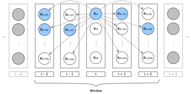
Figure 3: Each image in timestep t is compared to all images in other timesteps within the boundary of the sliding window W . After comparing all images of t , the sliding window is moved forward by one timestep.
